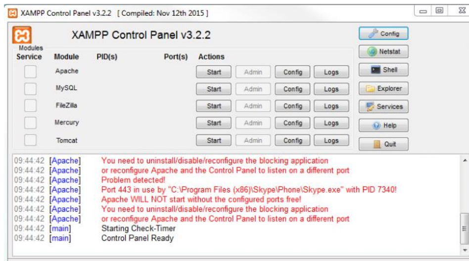
Figura 10: Panel XAMPP
